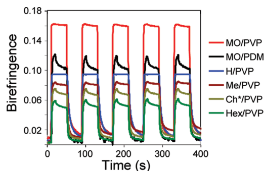
Figure 8. Inscription–relaxation–erasure cycles of photoinduced birefringence (PIB) in spin-coated films of the complexes.
