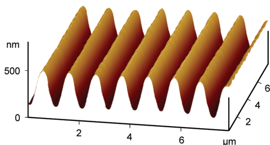
Figure 10. AFM surface profile of an optically inscribed SRG in a spin-coated film of MO/PVP exposed to a linearly polarized 488-nm Ar laser.
