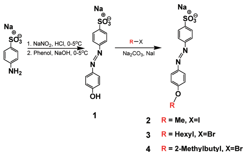
Scheme 2. Synthetic Route for the Chromophores a
