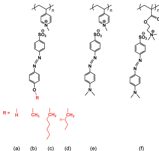
Scheme 1. Chemical Structures of the Complexes Studied a
