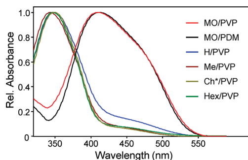
Figure 7. UV–visible spectra of spin-coated films of the complexes.
