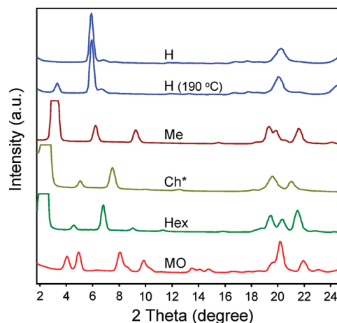
Figure 2. X-ray diffractograms of the Na + -neutralized chromophores at room temperature (unless otherwise indicated).
