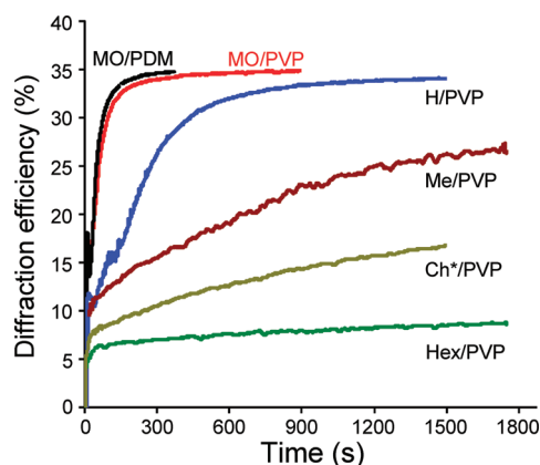
Figure 11. Diffraction efficiency during SRG inscription in spin-coated films of the complexes.
