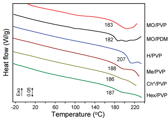
Figure 3. DSC thermograms of the complexes obtained during a second heating scan. The initial heating scan was to a maximum of 200 °C (180 °C for MO/PDM). The high temperature upturn in the MO/PVP thermogram is due to the onset of a sharp, intense exothermic peak related to the onset of degradation. 30 The numbers give the temperature in °C of the inflection point of the initial heat capacity change. 42
