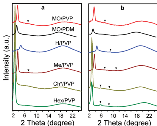
Figure 4. X-ray diffractograms of the complexes (a) at 160 °C (the maximum temperature in the heating–cooling cycle) and (b) at ambient temperature after cooling from 160 °C. Weak higher order diffraction peaks are indicated by arrows.
