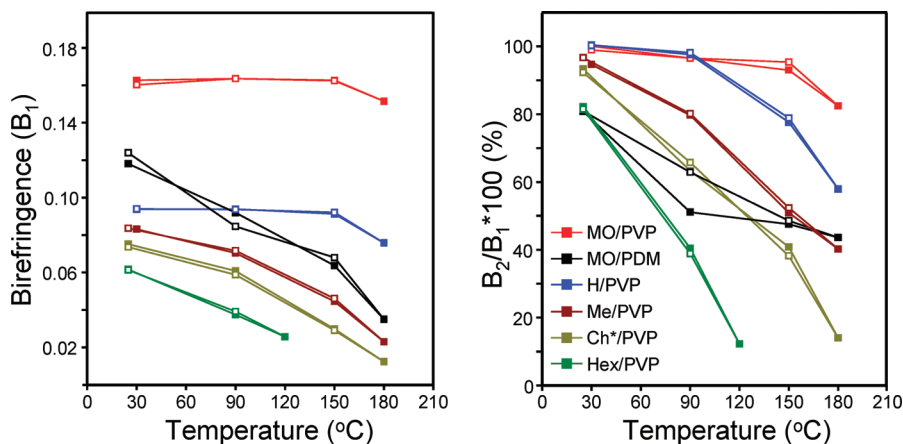
Figure 9. PIB of the different complexes as a function of temperature during heating (closed symbols) and cooling (open symbols): B_1 is the maximum PIB achieved at the end of the 10-s writing period, and B_2 is the birefringence remaining at the end of the 30-s relaxation period. For temperatures where closed symbols are not visible, they are coincident with the open symbols.
