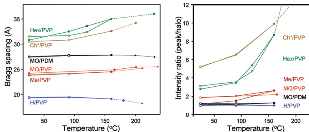
Figure 6. Bragg spacing and intensity (relative to the maximum intensity of the wide-angle halo) of the first order X-ray diffraction peak as a function of temperature for the complexes during heating (closed symbols) and subsequent cooling (open symbols). The temperatures below 160 °C for which only open symbols are visible have closed symbols coincident with the open ones. The points (lozenges) above 160 °C were obtained from a separate set of XRD experiments on samples heated up to degradation, with small lozenges indicating broadened, less intense peaks. The out-of-bound intensity ratios at the end of the dashed lines are 12.6 at 200 °C and 25.3 at 230 °C for Ch*/PVP and Hex/PVP, respectively.
