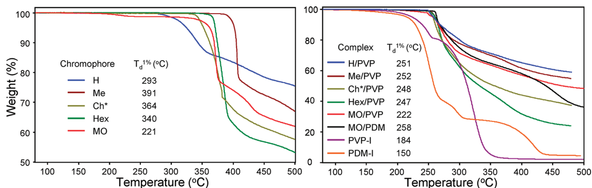
Figure 1. TGA thermograms (left) of the Na + -neutralized chromophores and (right) of the complexes and I - -neutralized polyelectrolytes.
