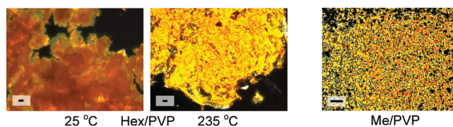
Figure 5. Polarizing optical micrographs for Hex/PVP in powder form at low and high temperature (left pair) and for a solution-cast film of Me/PVP (right). The scale bars represent 20 μm.
